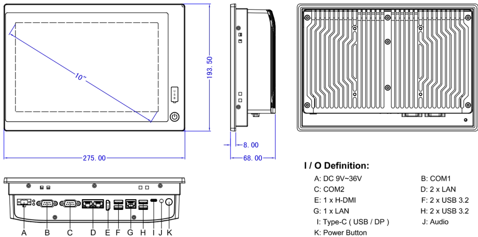
Panel Cutout Dimensions: 263 x 182 mm (10.35 x 7.16 in )
