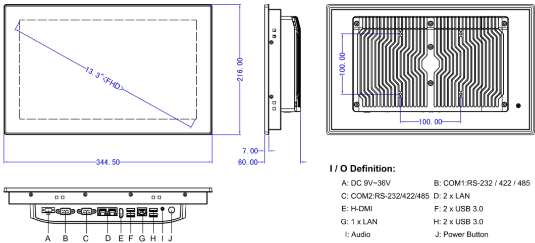
Panel Cutout Dimensions: 331 x 202 mm (13.03 x 7.95 in )
