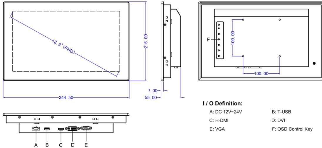
Panel Cutout Dimensions: 331 x 202 mm ( 13.03 x 7.95 in )
