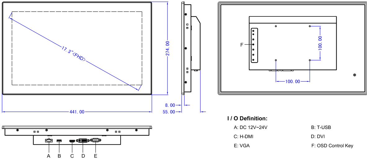
Panel Cutout Dimensions: 427 x 260 mm (16.82 x 10.24 in)
